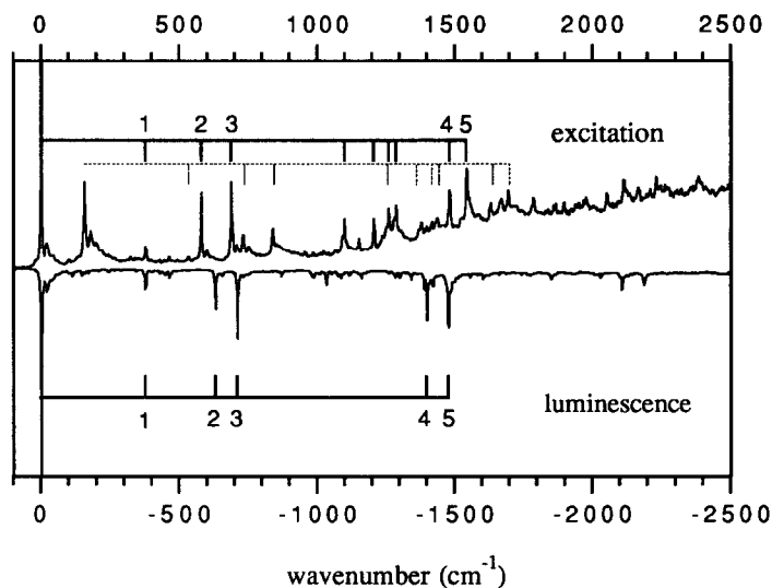
Figure 1. Excitation and luminescence spectra at 5 K of the [ThpyBpy] doped mixed crystal. The spectra are drawn so that the common origins coincide and the vibrational sideband structure can be compared.
